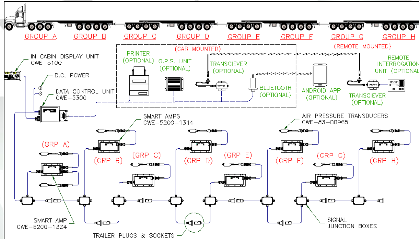
Typical eight channel CHEK-WAY® Eliminator configuration
